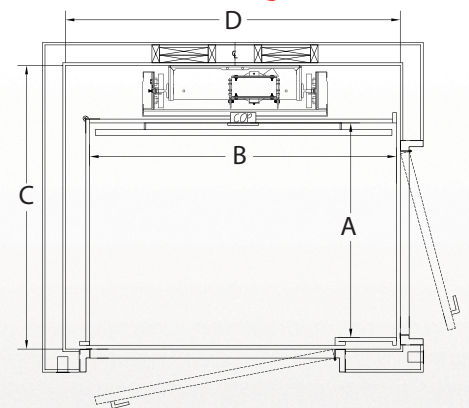
90° Exit Configuration
